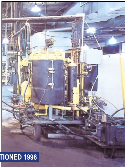
ADMIRAL POLYOL ISOCYANATE FOAM APPLICATION SYSTEM
